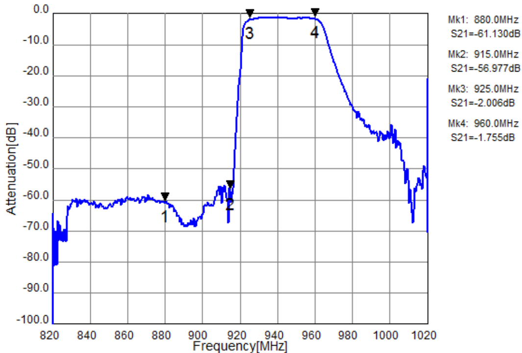
Figure 4-1. Electrical Characteristics
