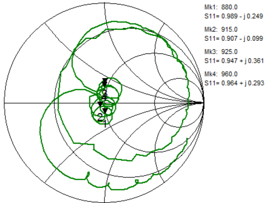
Figure 4-5. Electrical Characteristics
