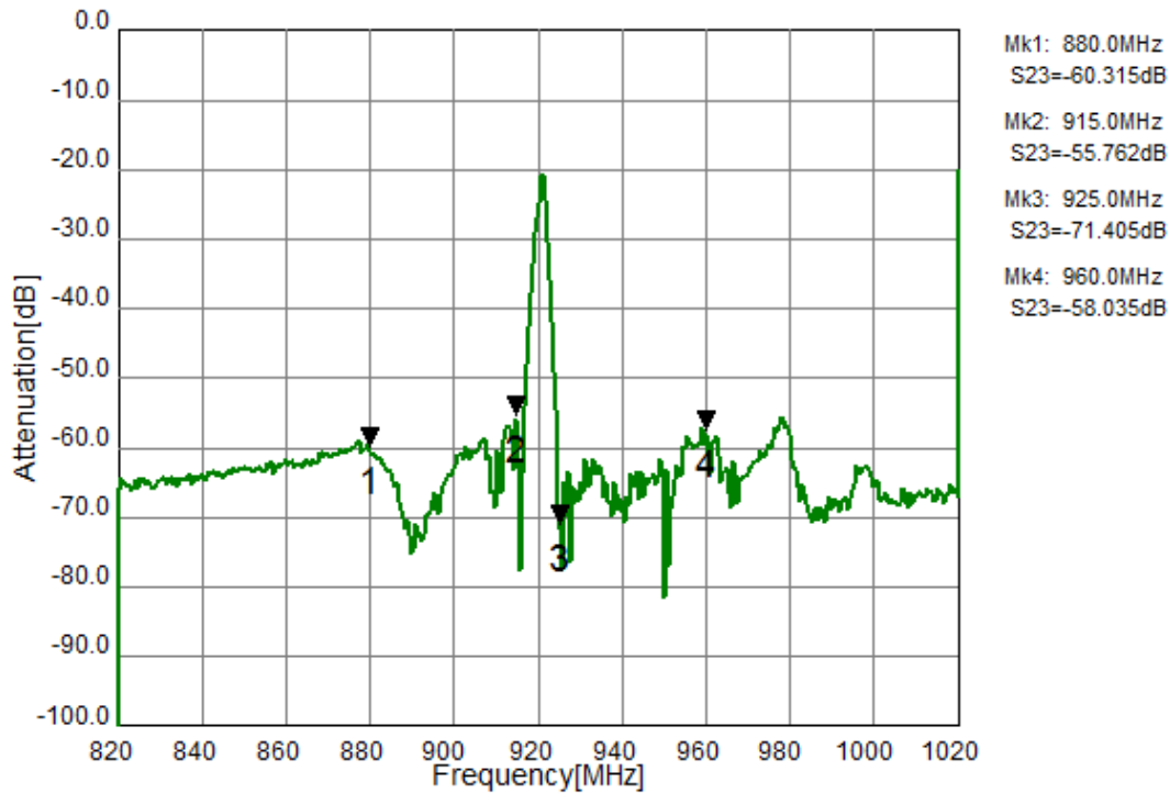
Figure 4-2. Electrical Characteristics
